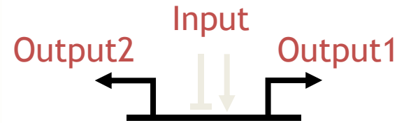
Figure 1. The phage lysis-lysogeny decision circuit. (a) Bold horizontal lines indicate stretches of double-stranded DNA. Arrows over genes indicate direction of transcription. Dashed boxes enclose operator sites that comprise a promoter control complex. The three operator sites, OR1-3 , of the "lambda switch" implement concentration-dependent logic controlling promoters PRM and PR . Cro and CII dimers bind to the three sites with different affinities and in opposite order to control the activation level of the PRM and PR promoters (PTASHNE 1992; SHEA and ACKERS 1985). The five boxes R1-R5 contain nongenetic protein reaction subsystems. In R1, R2, and R5, "deg" indicates degradation. When protein N is available, transcribing RNAPs can be antiterminated at the NUTR and NUTL sites; termination sites TR1 and TL1 are inoperative for antiterminated RNAPs. The CII dimer acts as either a repressor or activator of promoter PRM , depending on its concentration. See text for discussion of the proteases labeled as P1 and P2 in R3 and R4. (b) decision circuit DNA organization. Phage-encoded genetic elements of the decision circuit are located in a 5000 nucleotide region of the phage DNA. Genes are separated onto leftward and rightward transcribed strands as indicated by the arrows. Rightward extensions of the antiterminated PR transcript transcribe the O and P genes essential for phage genome replication and the Q gene that controls transcription of later genes on the lytic pathway. Leftward extension of the antiterminated PL transcript transcribes xis and int genes essential for phage chromosome integration and excision into and out of the host chromosome. Locations of four termination sites are indicated by TR1-2 and TL1-2 .
