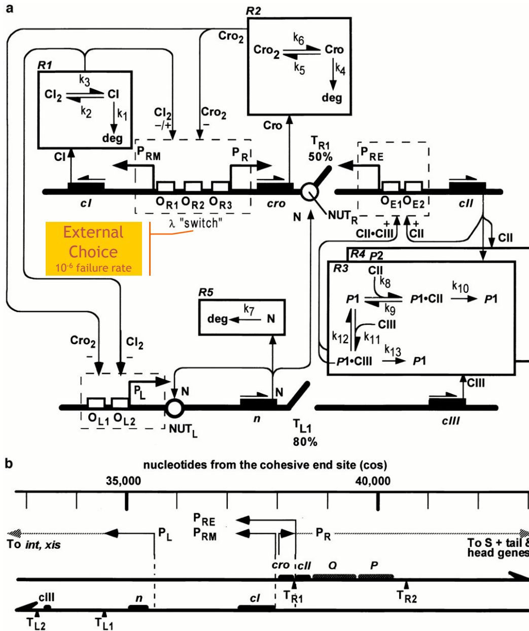
Figure 1. The phage lysis-lysogeny decision circuit. (a) Bold horizontal lines indicate stretches of double-stranded DNA. Arrows over genes indicate direction of transcription. Dashed boxes enclose operator sites that comprise a promoter control complex. The three operator sites, OR1-3 , of the "lambda switch" implement concentration-dependent logic controlling promoters PRM and PR . Cro and CII dimers bind to the three sites with different affinities and in opposite order to control the activation level of the PRM and PR promoters (PTASHNE 1992; SHEA and ACKERS 1985). The five boxes R1-R5 contain nongenetic protein reaction subsystems. In R1, R2, and R5, "deg" indicates degradation. When protein N is available, transcribing RNAPs can be antiterminated at the NUTR and NUTL sites; termination sites TR1 and TL1 are inoperative for antiterminated RNAPs. The CII dimer acts as either a repressor or activator of promoter PRM , depending on its concentration. See text for discussion of the proteases labeled as P1 and P2 in R3 and R4. (b) decision circuit DNA organization. Phage-encoded genetic elements of the decision circuit are located in a 5000 nucleotide region of the phage DNA. Genes are separated onto leftward and rightward transcribed strands as indicated by the arrows. Rightward extensions of the antiterminated PR transcript transcribe the O and P genes essential for phage genome replication and the Q gene that controls transcription of later genes on the lytic pathway. Leftward extension of the antiterminated PL transcript transcribes xis and int genes essential for phage chromosome integration and excision into and out of the host chromosome. Locations of four termination sites are indicated by TR1-2 and TL1-2 .
